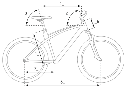
MERCEDES-BENZ FITNESS BIKE 29"
